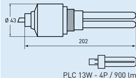
PLC 13W - 4P / 900 lm
