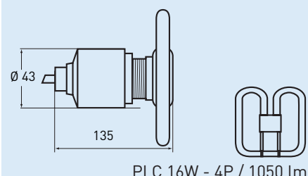
PLC 16W - 4P / 1050 lm
